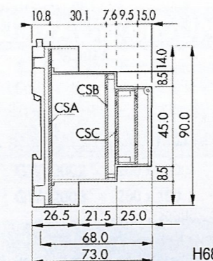
Top Plate for H53/H68
