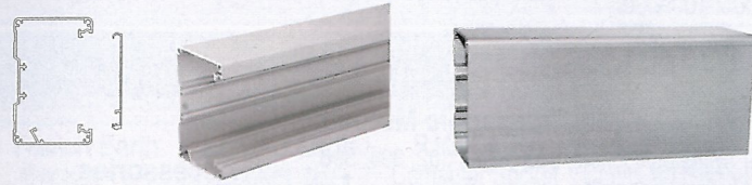
Aluminium Power Skirting - 105 x 65mm Finish: Natural Anodised
