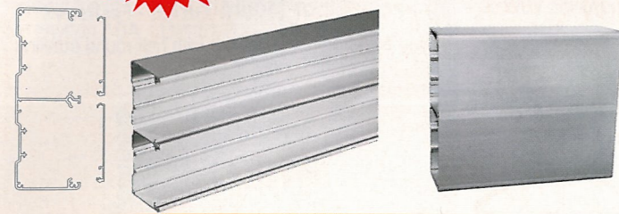
Aluminium Power Skirting - 180 x 65mm Finish: Natural Anodised
